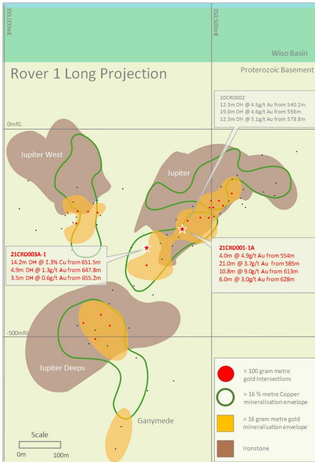
Figure 1: Rover 1 long projection showing 21CRD001-1A and 21CRD003A-1, mineralisation and historic gold intersection points.
