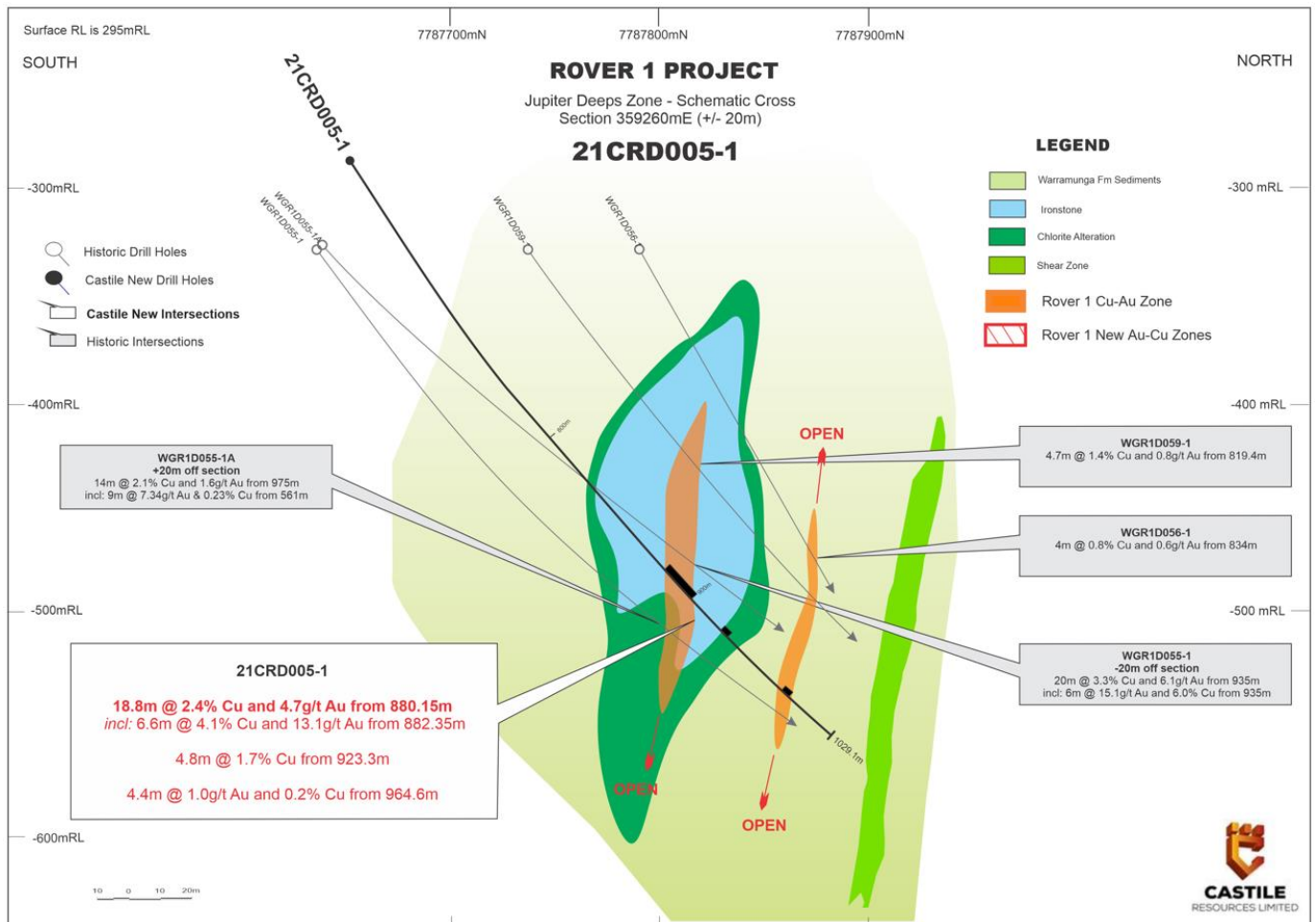
Figure 1: Schematic Cross Section of Hole 21CRD005-1
