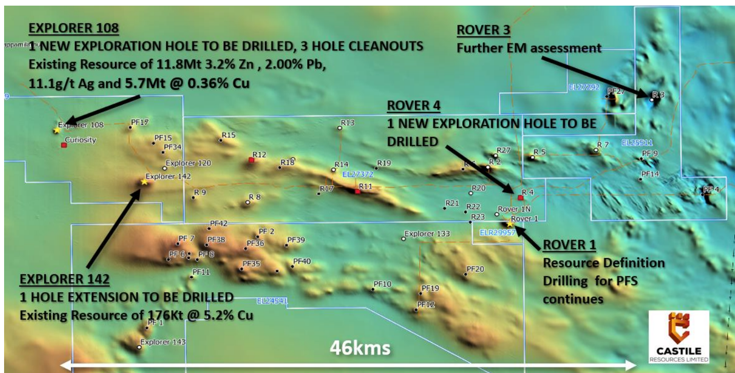
Figure 1: Map of Castile's Rover Mineral Field Prospects
