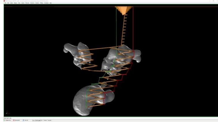
Proposed mining shapes for magnetite, gold and copper
