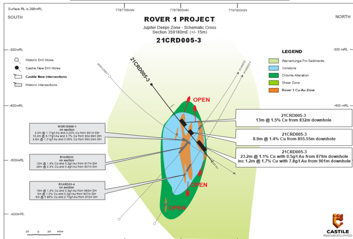
Figure 1: Schematic Cross Section of Hole 21CRD005-3
