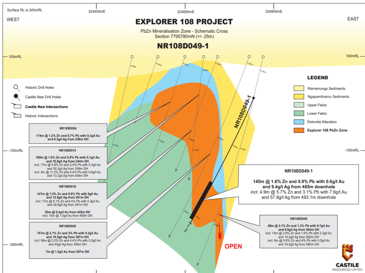
Figure 1: Schematic Cross Section of Explorer 108 Hole NR108D049-1
